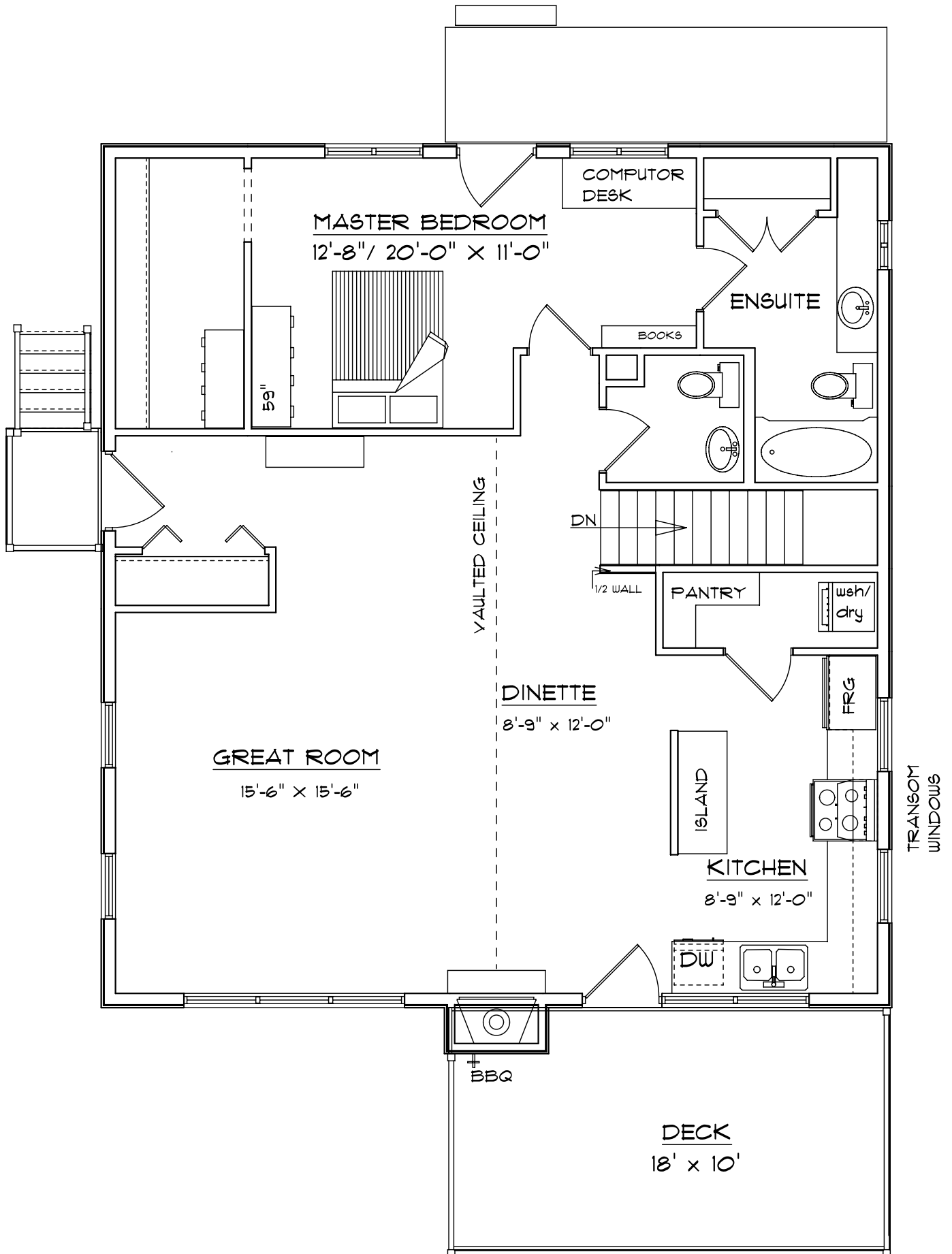
MAIN FLOOR PLAN 1129 sq.ft.
